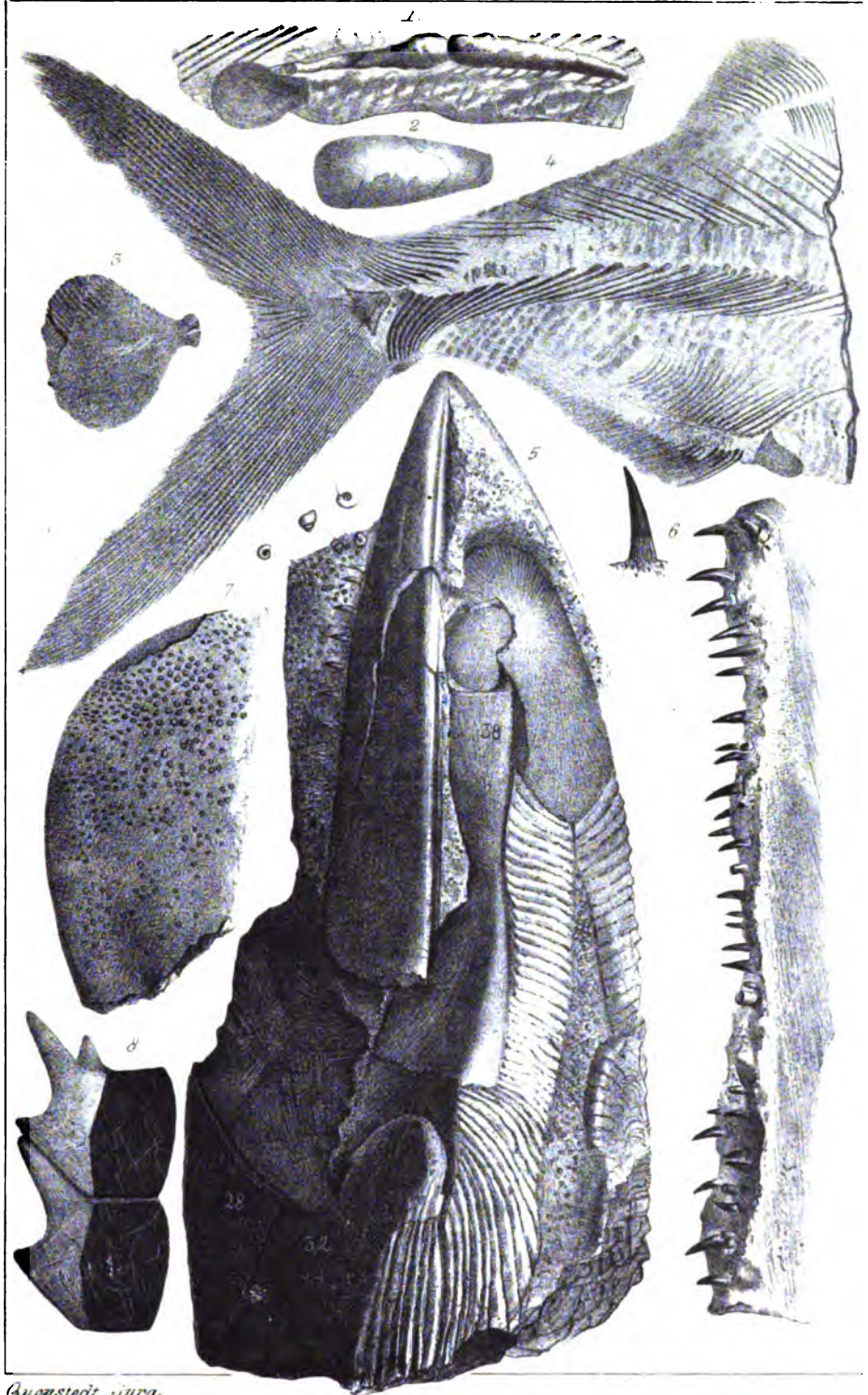
Quonstedt nura
